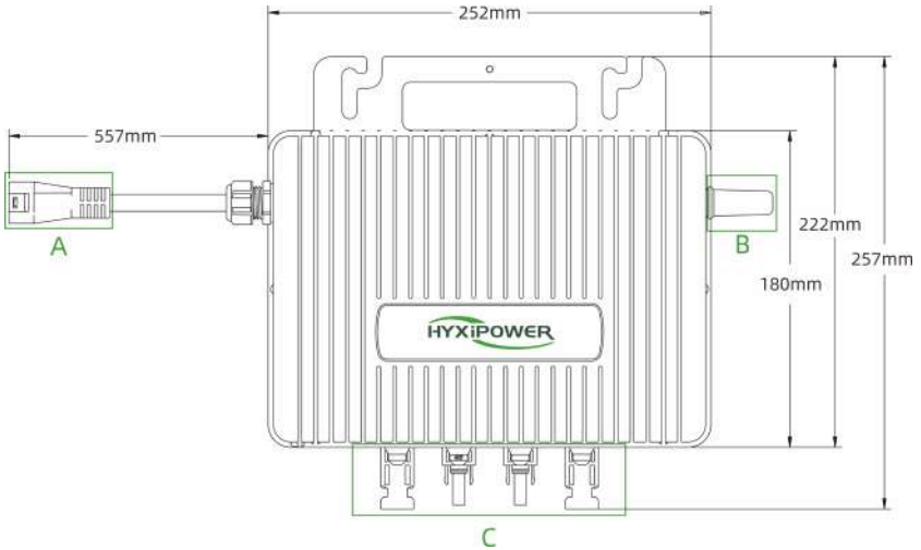
A: AC Branch Connector
