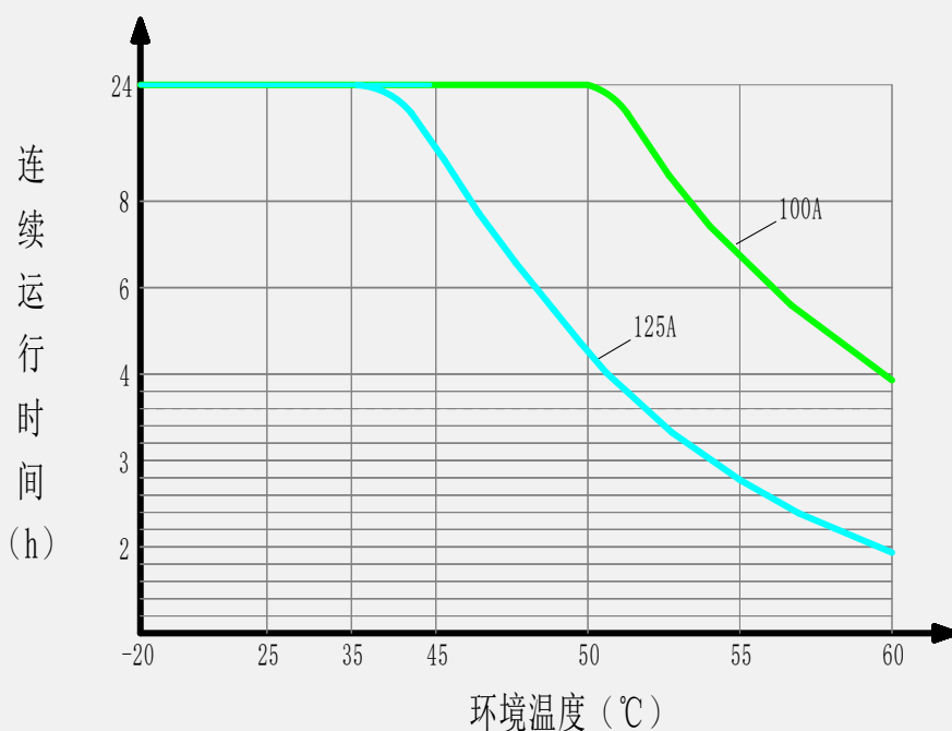
图/ Figure2 3U RBMS 环温与运行时间曲线图-Curve of Environmental Temperature and Operating Time
